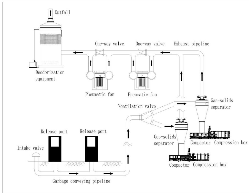
Figure 1. Working principle the pneumatic waste conveying system
