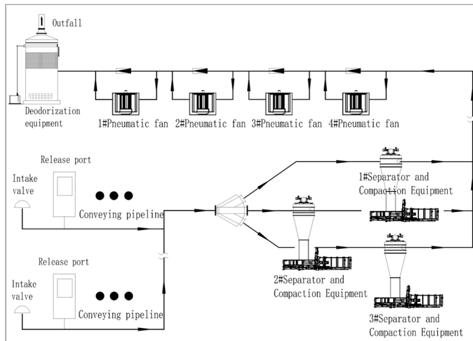
Figure 4. Process flow diagram of the pneumatic waste conveying system in non-storage mode
