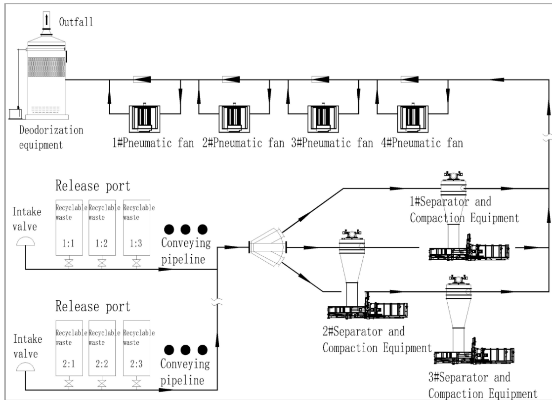
Figure 5. Process flow diagram of the pneumatic waste conveying system in storage-enabled mode
