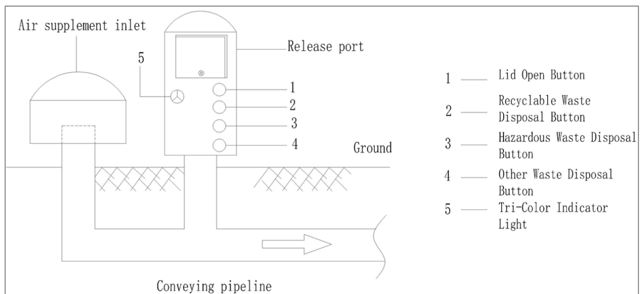
Figure 2. Schematic diagram of a non-storage waste inlet
