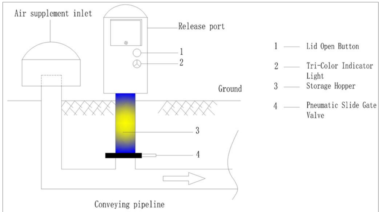
Figure 3. Schematic diagram of a storage-enabled waste inlet
