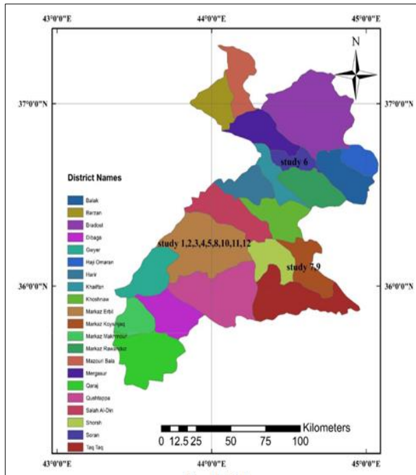
Figure 4. Groundwater quality investigation locations (Hawezi et al., 2020)
